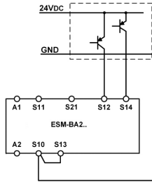
Fig. 9: Dual-channel emergency stop circuit with pnp semiconductor outputs/OSSD outputs with short circuit detection (category 4, up to PL e).
