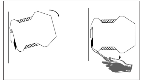
Fig. 2: Mounting/removing
