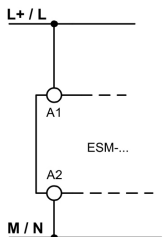
Fig. 15: Connection of the power supply to terminals A1 and A2 (power supply according to the technical data).
