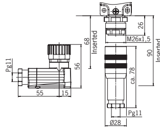
Fig. 11: Dimension drawing for NZ2VZ5... with plug connector SR11
