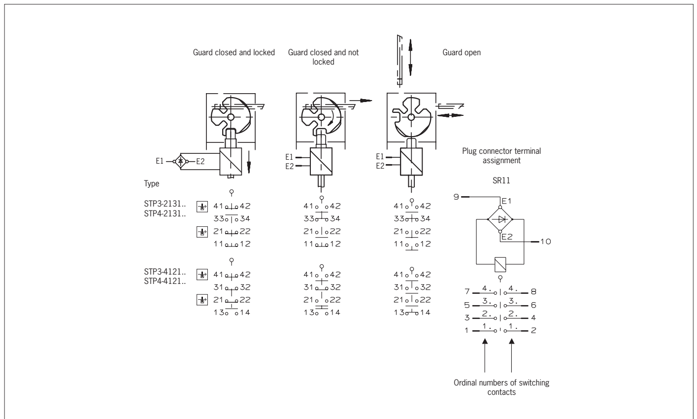
Fig. 3: Switching elements and switching functions
