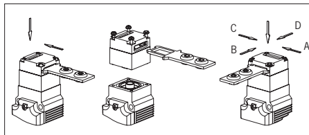
Fig. 1: Changing the actuating direction
