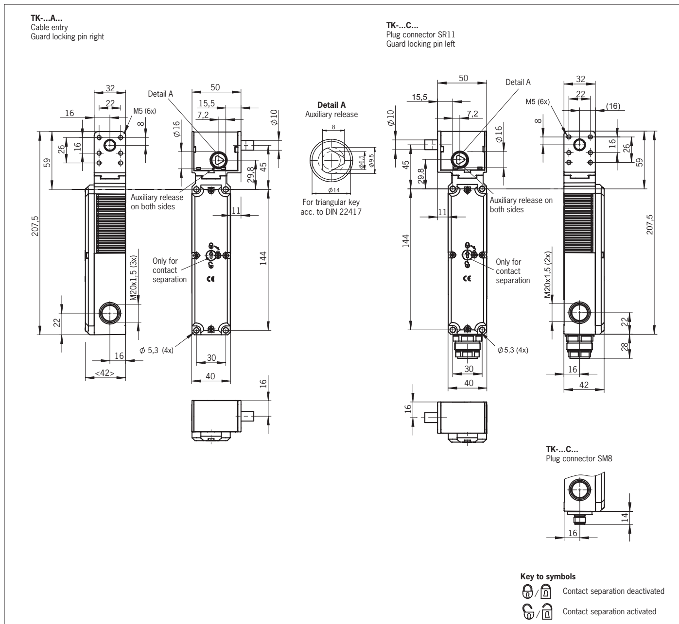
Fig. 3: Dimension drawing
