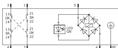
TZ...045177/045181/048492 (with plug connector SR6)
