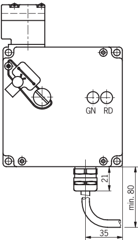
TZ...C1527 with connecting cable
