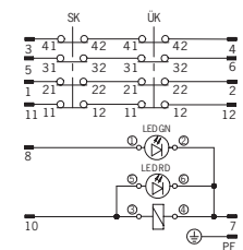
TZ..BHA...RC2408 (with plug connector BHA12)
