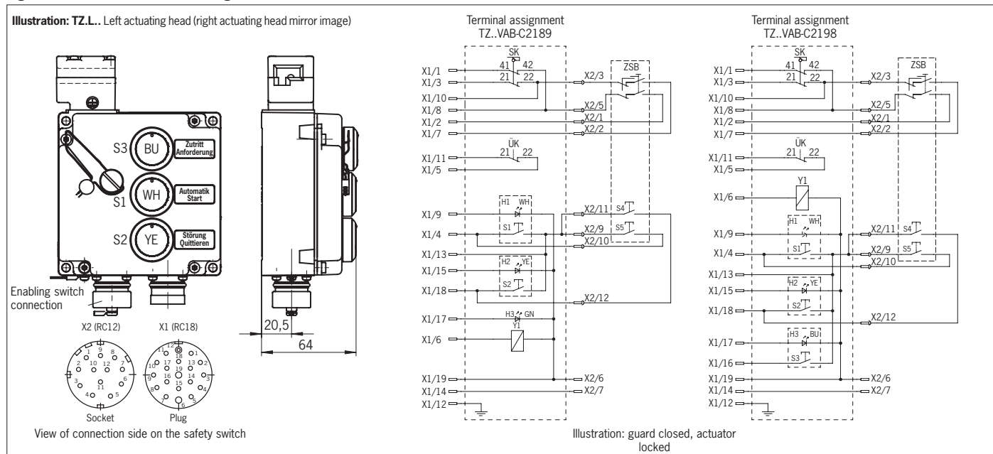
Fig. 8: TZ..VAB-C2189/2198 with lamps/illuminated pushbuttons and enabling switch connection
