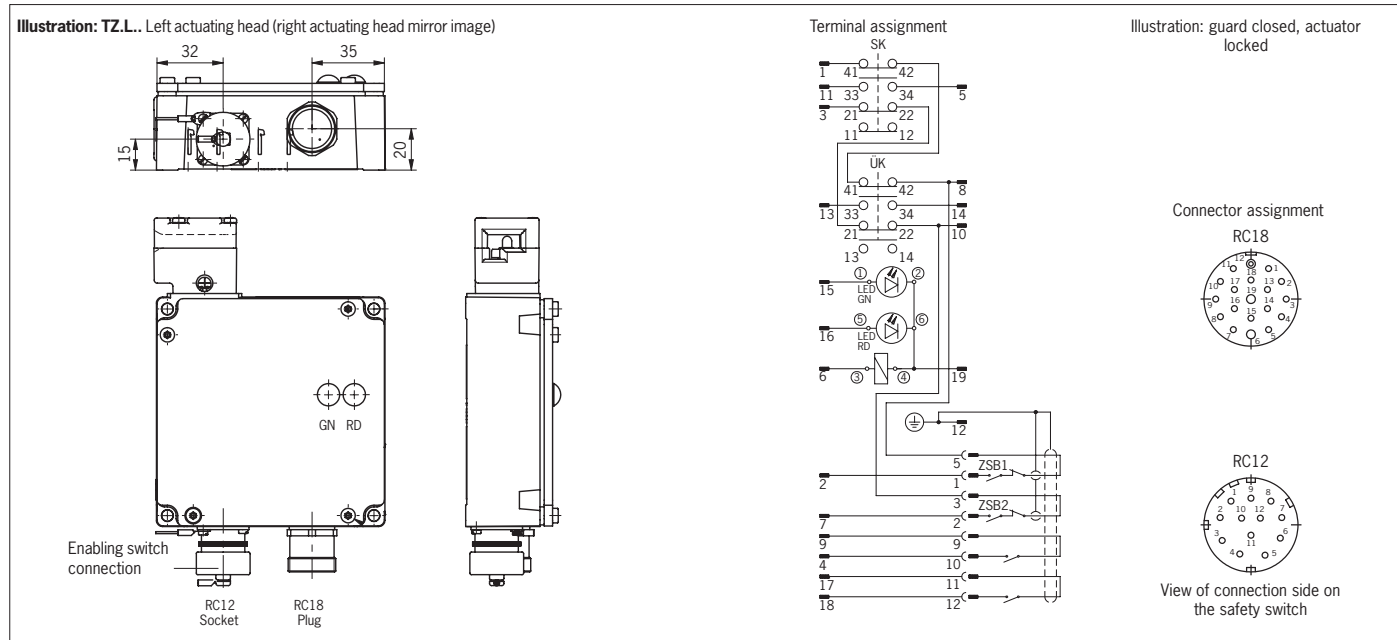
Fig. 7: TZ..VAB-C1803 with enabling switch connection
