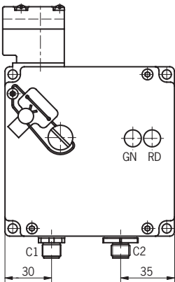
TZ...C1888 with plug connectors 2 x M12
