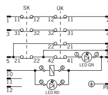
TZ..BHA...RC1924 (with plug connector BHA12)
