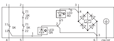
TZ..C1527 (with connecting cable)
