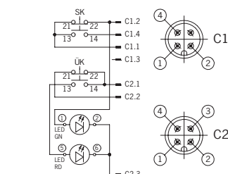
TZ.SEM4-C1888 (with plug connectors 2 x M12 according to DESINA)
