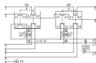
TZ..BHA...C1781 (with plug connector BHA12)
