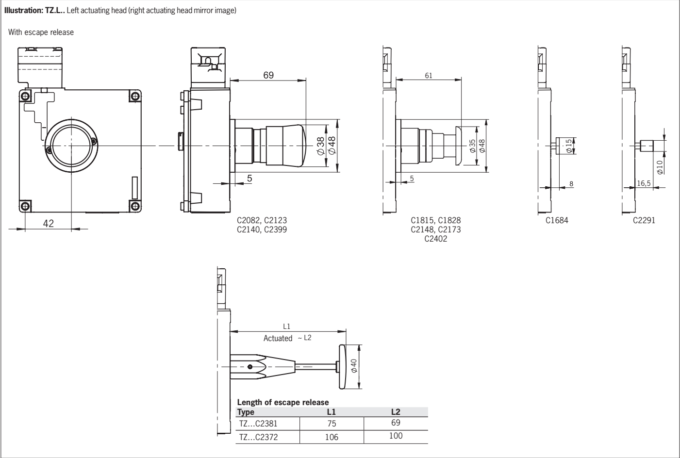
Fig. 4: Dimension drawings for escape releases
