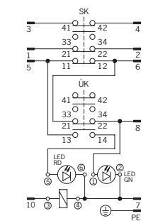
TZ..VABL12C-MF (with plug connector BHA12)
