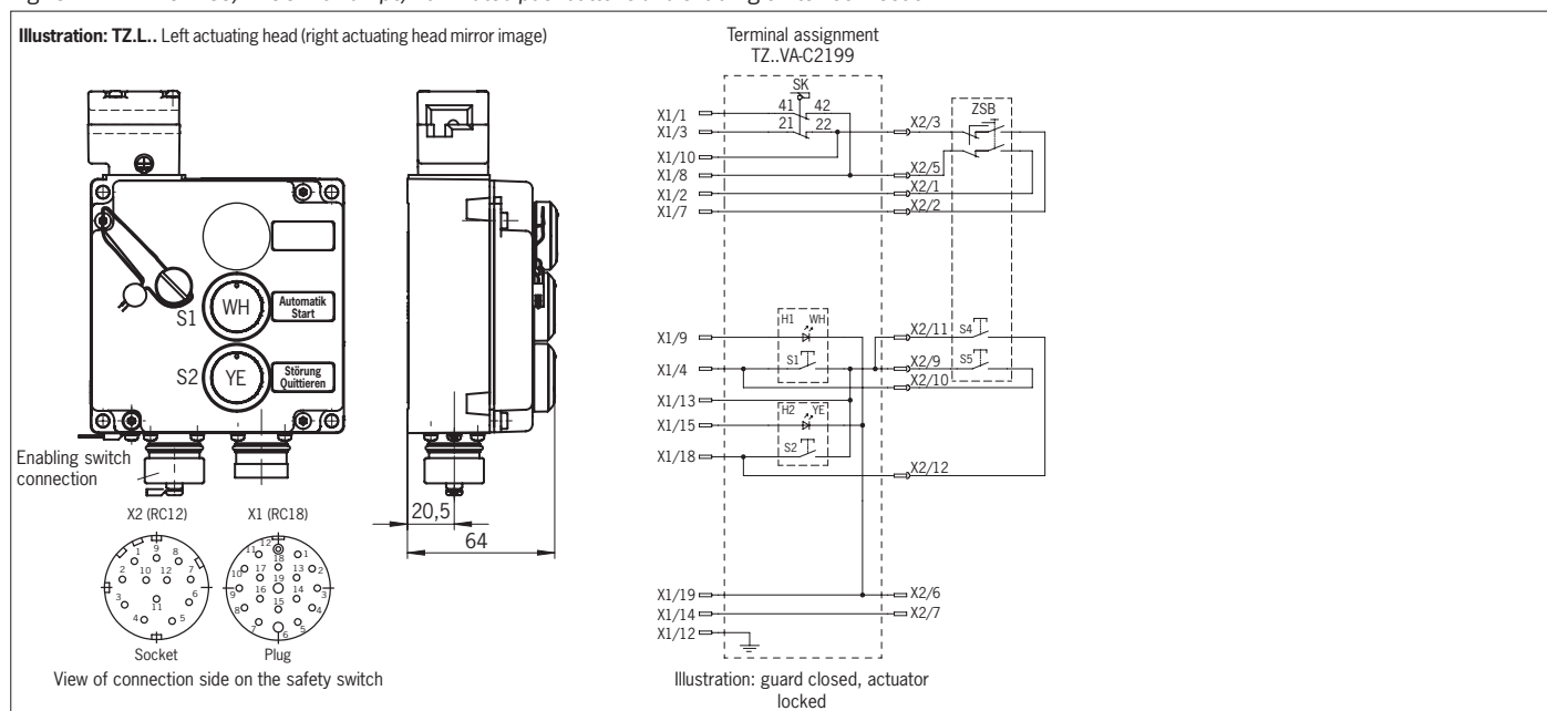
Fig. 9: TZ..VA-C2199 with illuminated pushbuttons and enabling switch connection
