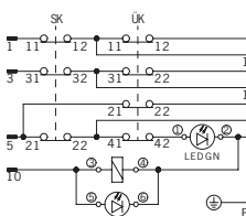
TZ..BHA...C1902 (with plug connector BHA12)
