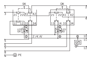
TZ..BHA...C1781 (con conector BHA12)
