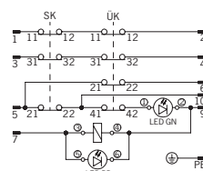
TZ..BHA...C1903/C2148/C2399 (with plug connector BHA12)
