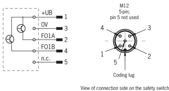
Figure 2: Connector assignment of safety switch CES-I-BP-...-SI
