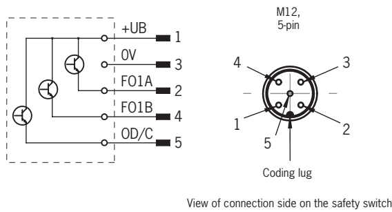
Figure 1: Connector assignment of safety switch CES-I-BP-...-SB
