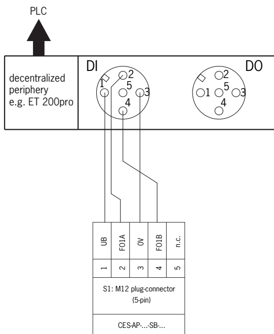
Figure 3: Connection example for connection to decentralized peripheral systems
