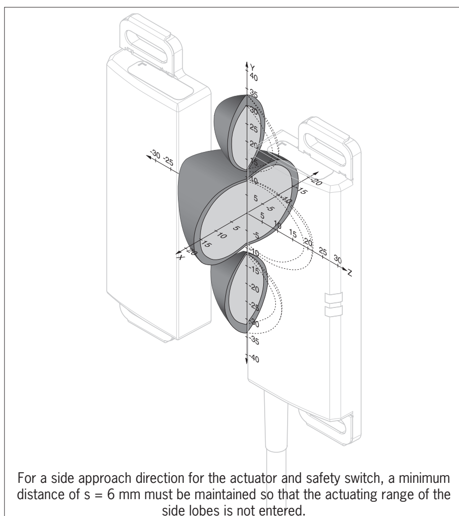
Figure 4: Typical actuating range
