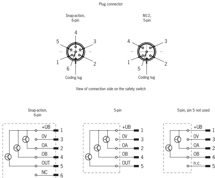
Figure 1: Connector assignment of safety switch CES-AP-C.2
