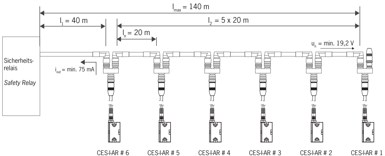
Fig. 1: Circuit example with six CES-I-AR
