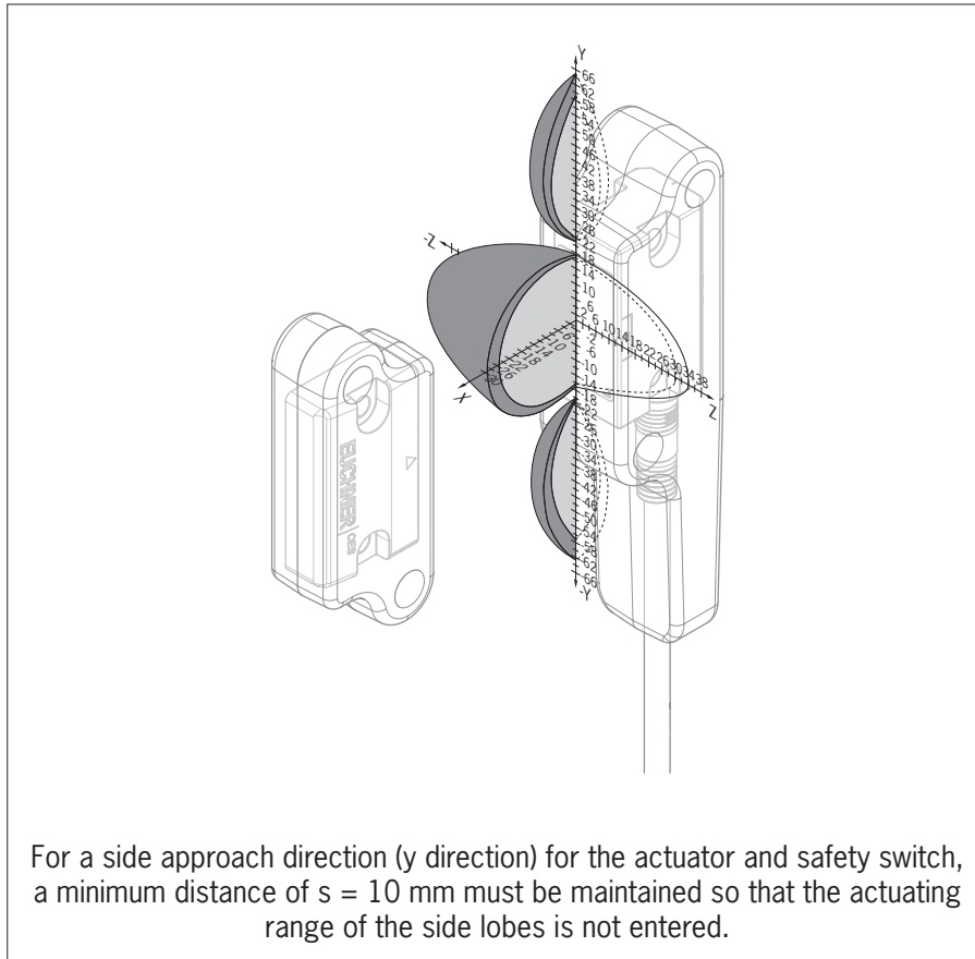
Fig. 7: Typical operating distance
