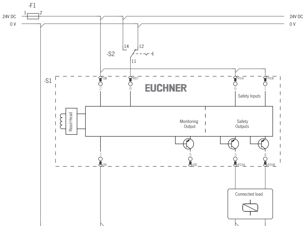
Fig. 3: Connection example for separate operation of a CES-I-AR...
