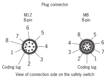
Fig. 2: Connector assignment of safety switch CES-I-AR
