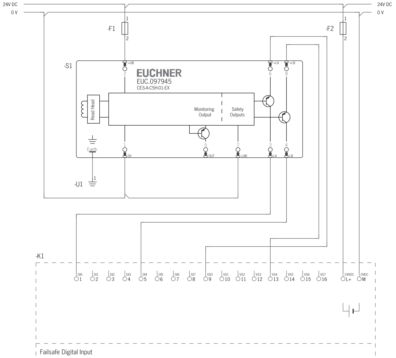
Fig. 2: Connection example for CES-A-C5H-01-EX
