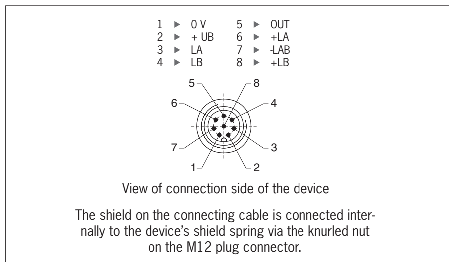
Fig. 1: Connector assignment of safety switch CES-A-C5H-01-EX
