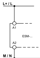
Fig. 9: Connection of the power supply to terminals A1 and A2 (power supply according to the technical data).
