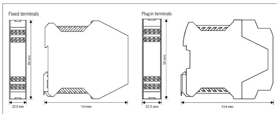
Fig. 4: Dimension drawing for ESM-ES3..
