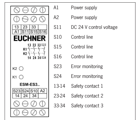
Fig. 3: Connections
