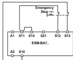
Fig. 5: Dual-channel emergency stop circuit with short circuit and ground fault monitoring (category 4, up to PL e).
