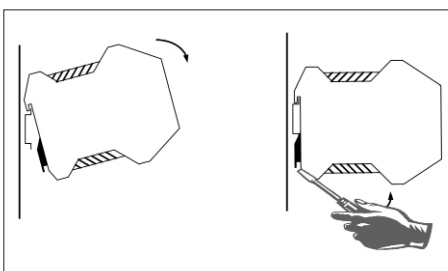
Fig. 1: Mounting/removing
