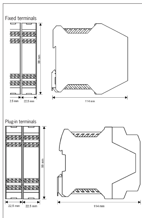
Fig. 2: Dimension drawing for ESM-BA7..
