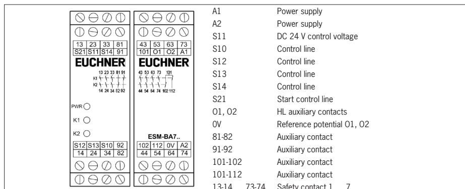
Fig. 4: Connections
