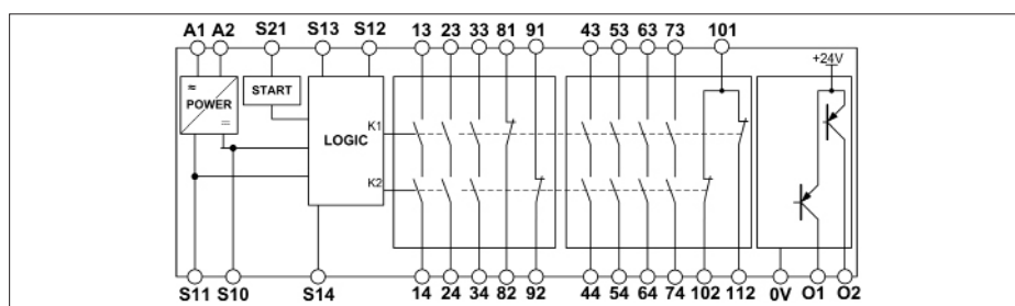
Fig. 3: Block diagram for ESM-BA7..
