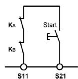
Fig. 12: Feedback loop. Monitoring of externally connected contactors or expansion modules.
