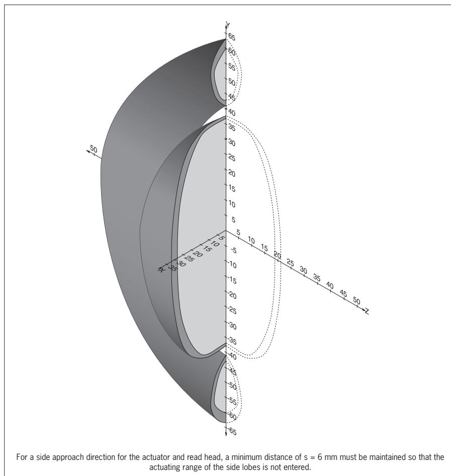
Figure 4: Typical actuating range
