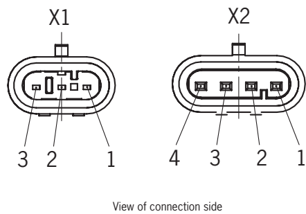
Figure 1: Connector assignment of safety switch CES-AH
