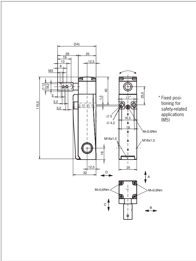
Fig. 5: Dimension drawing for NM11AK / NM02AK / NM12AK / NM03AK
