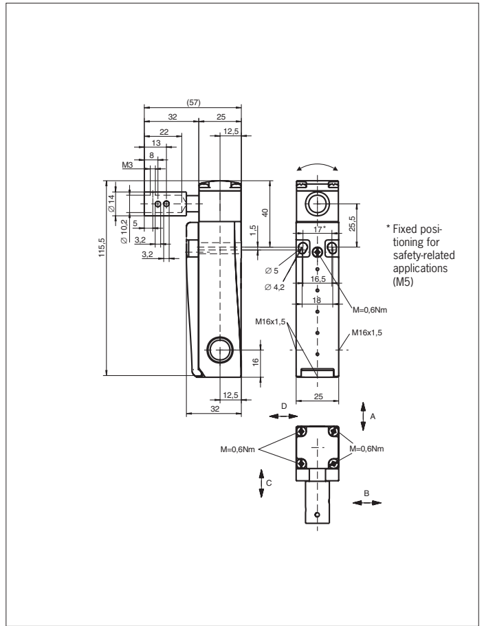
Fig. 6: Dimension drawing for NM11AG / NM02AG / NM12AG / NM03AG
