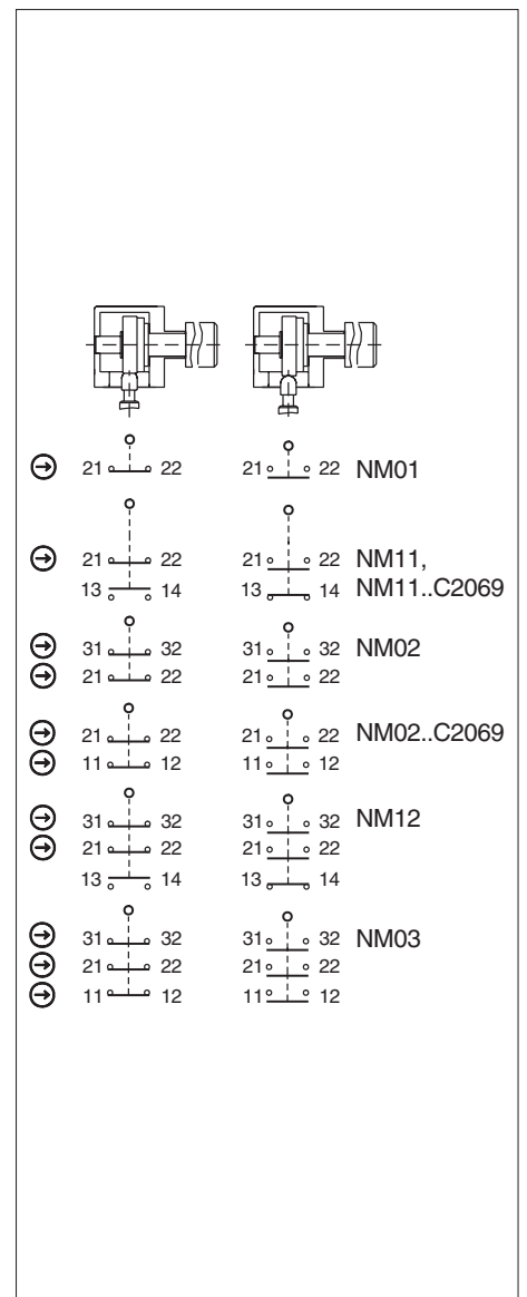
Fig. 3: Switching elements and switching functions
