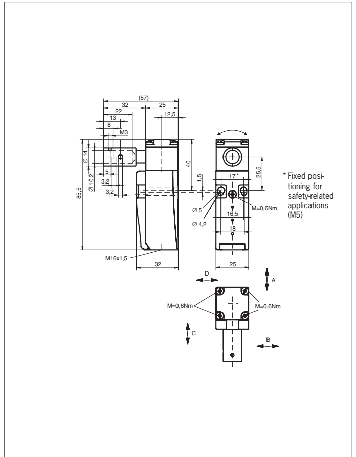
Fig. 8: Dimension drawing for NM01AG, NM..AG..C2069
