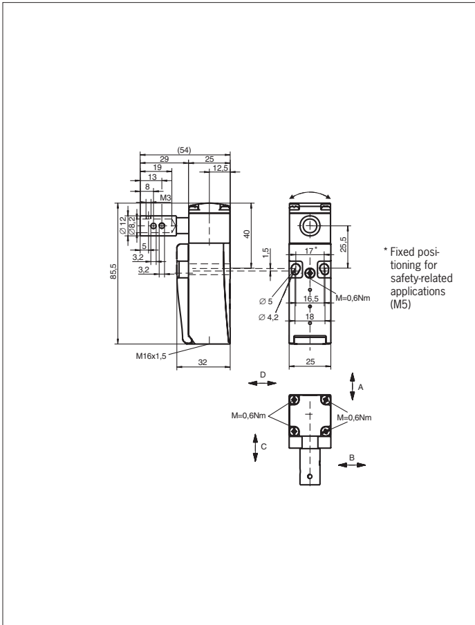
Fig. 7: Dimension drawing for NM01AK, NM..AK..C2069
