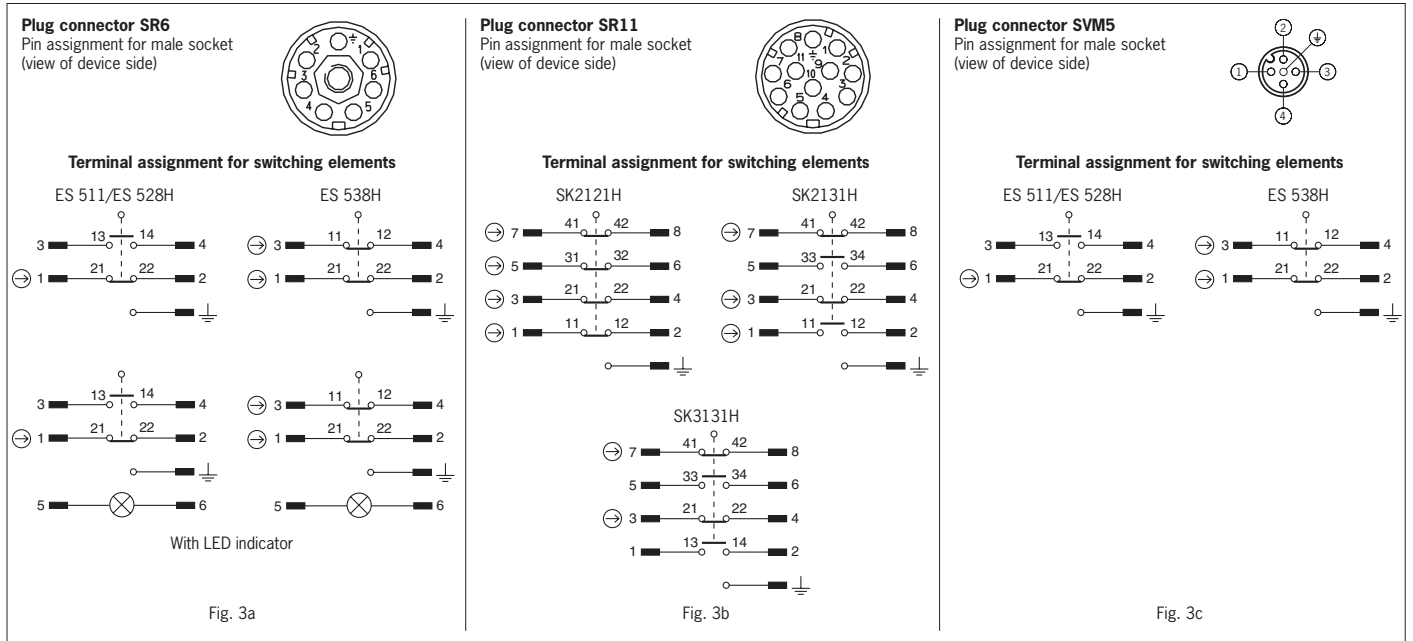
Fig. 3: Switching elements and connector assignment
