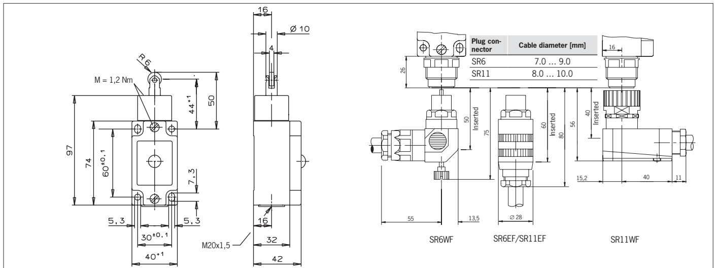
Fig. 4: Dimension drawing for NZ1... with cable entry and NZ2... with plug connector
