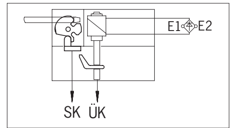
Fig. 1: Function of safety switch STM Pro
