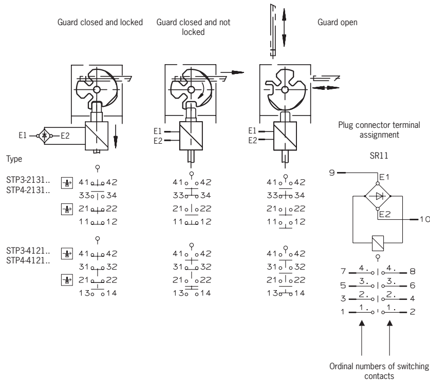
Fig. 3: Switching elements and switching functions
