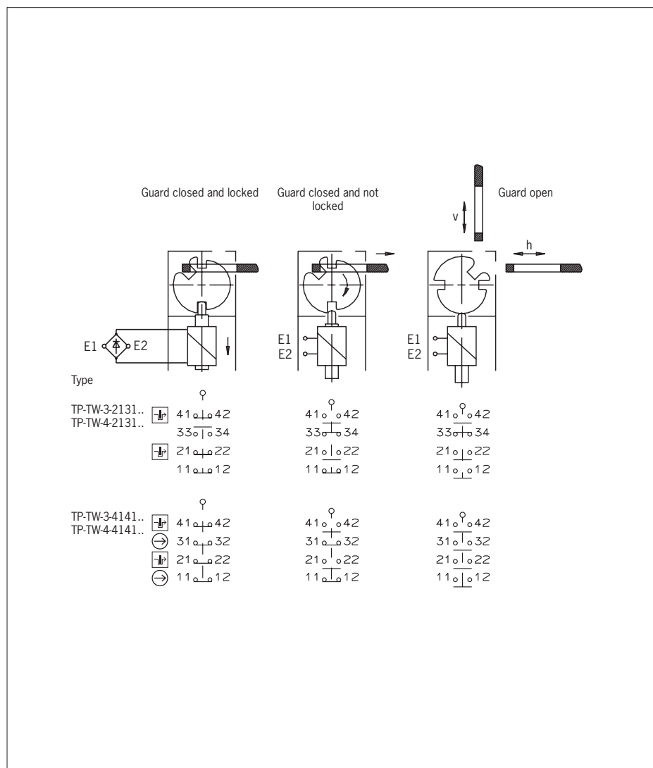
Fig. 4: Switching elements and switching functions
