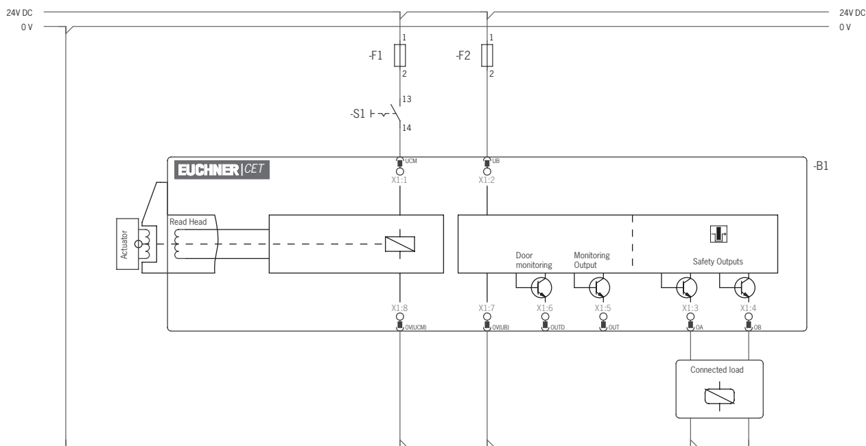
Figure 7: Wiring diagram C/D, CET 3/4-AP with plug connector 1 x M12, with monitoring output OUT or DIA on X1:5 Single-channel control of the guard locking solenoid
