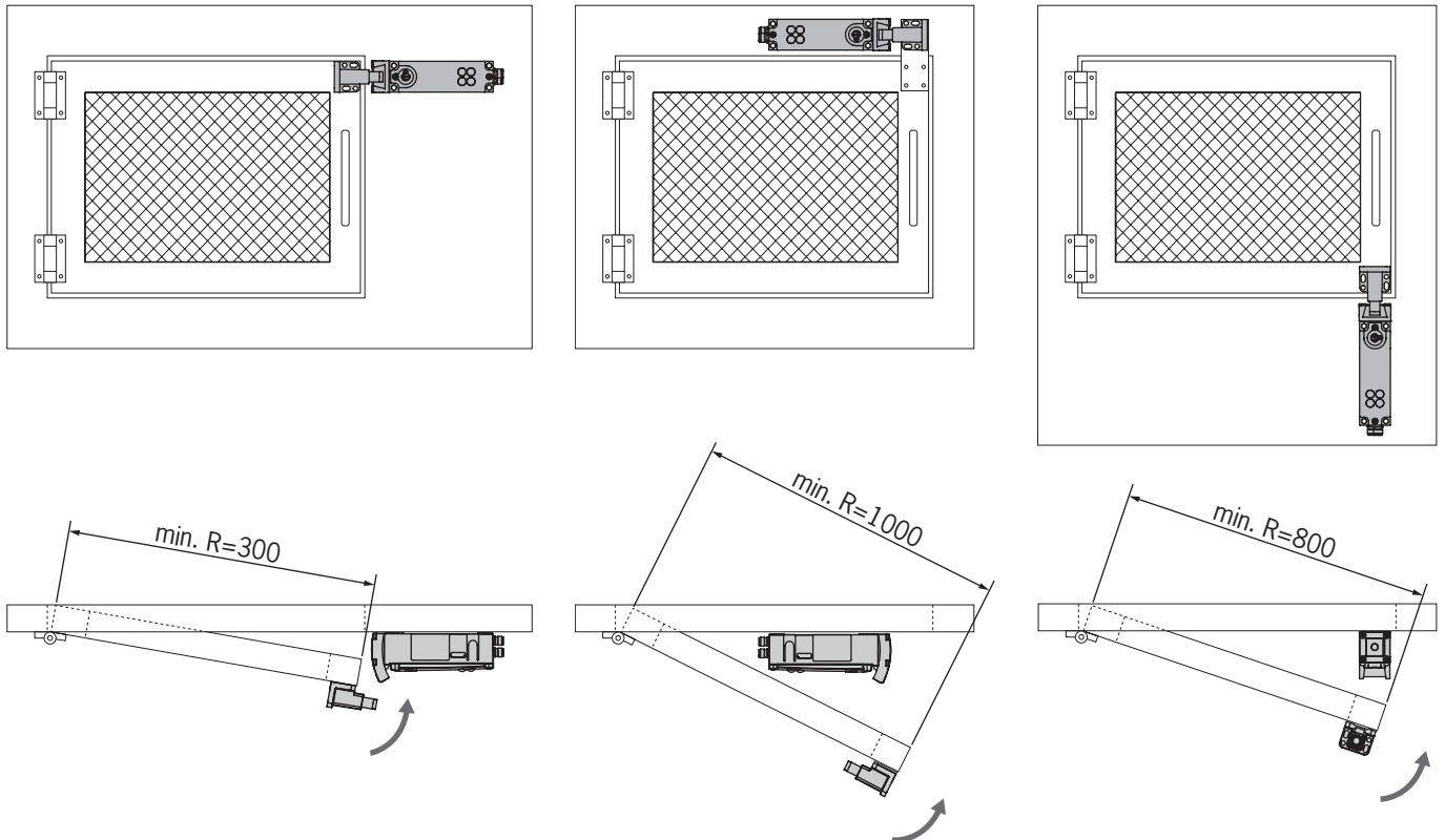
Figure 2: Installation situation and door radii
