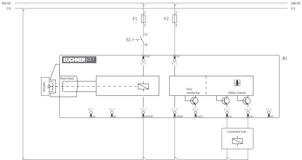
Figure 5: Wiring diagram B, CET 3/4-AP with plug connector 2 x M12, with door monitoring output Single-channel control of the guard locking solenoid
