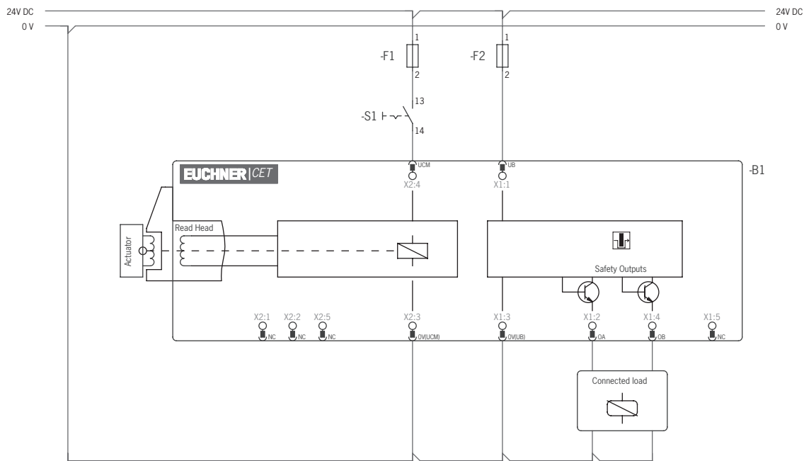
Figure 3: Wiring diagram A, CET 3/4-AP with plug connector 2 x M12, without door monitoring output Single-channel control of the guard locking solenoid
