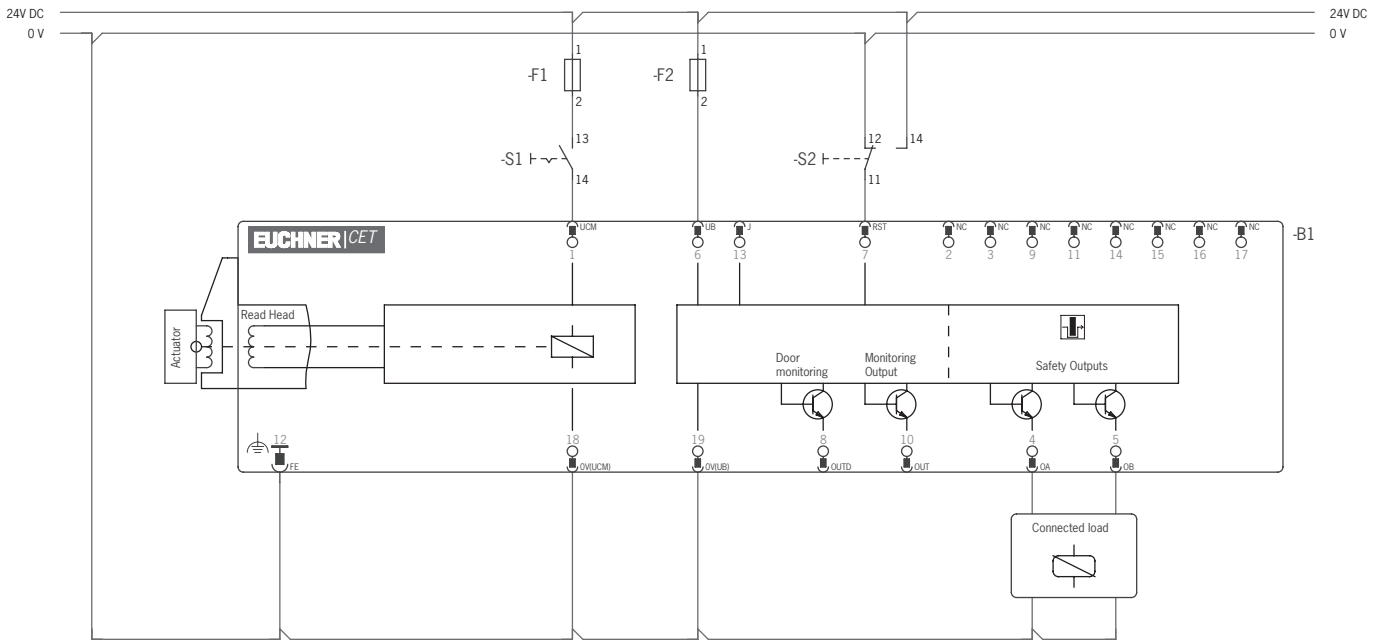
Figure 9: Wiring diagram E, CET 3/4-AP with plug connector 1 x M23 Single-channel control of the guard locking solenoid
