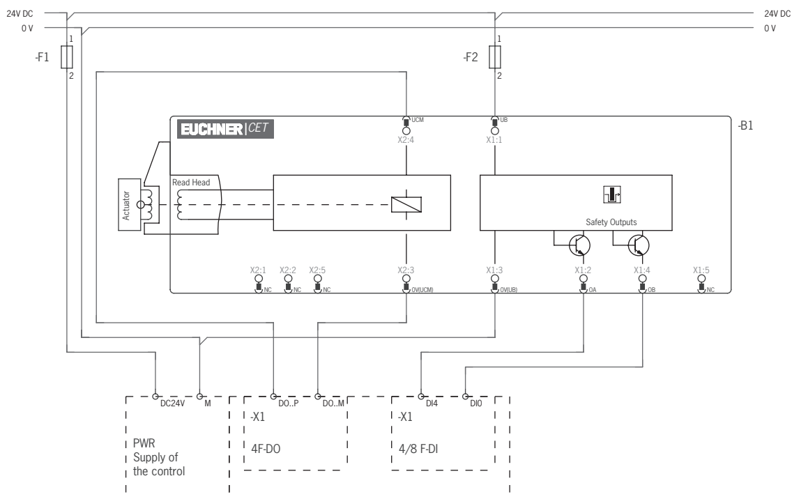
Figure 4: Wiring diagram A, CET 3/4-AP with plug connector 2 x M12, without door monitoring output Dual-channel control of the guard locking solenoid
