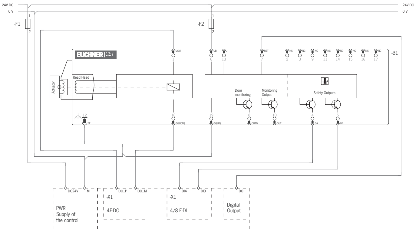
Figure 10: Wiring diagram E, CET 3/4-AP with plug connector 1 x M23 Dual-channel control of the guard locking solenoid
