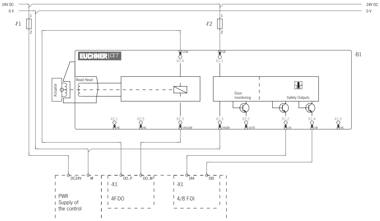
Figure 6: Wiring diagram B, CET 3/4-AP with plug connector 2 x M12, with door monitoring output Dual-channel control of the guard locking solenoid
