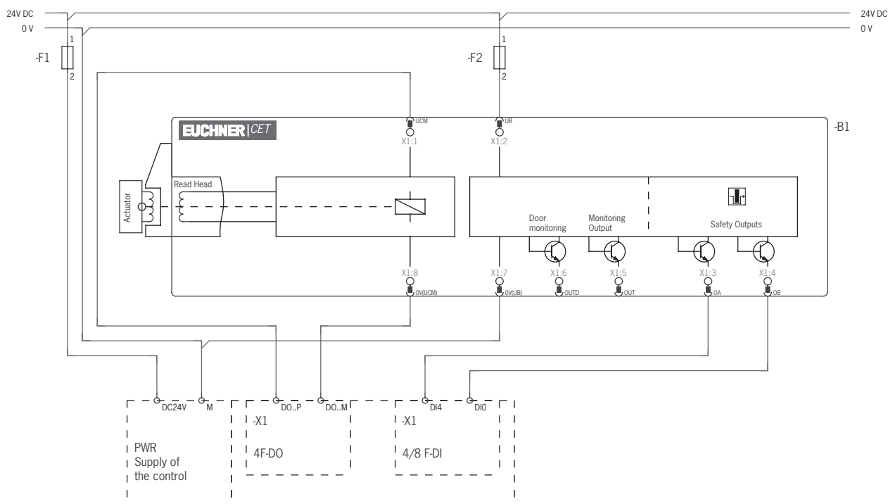
Figure 8: Wiring diagram C/D, CET 3/4-AP with plug connector 1 x M12, with monitoring output OUT or DIA on X1:5 Dual-channel control of the guard locking solenoid
