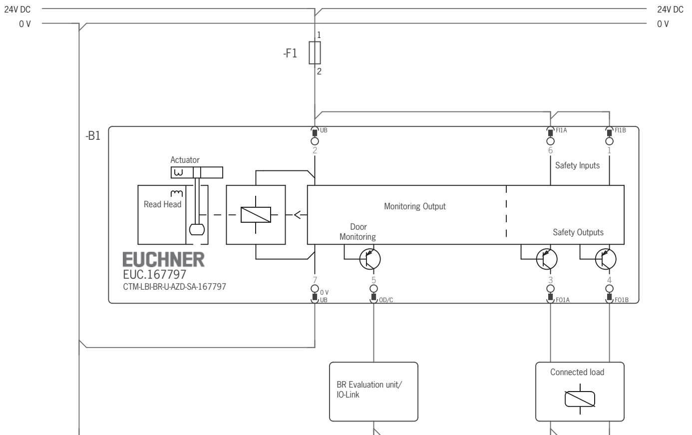
Fig. 1: Connection example with control of guard locking via IO-Link (principle of operation)
