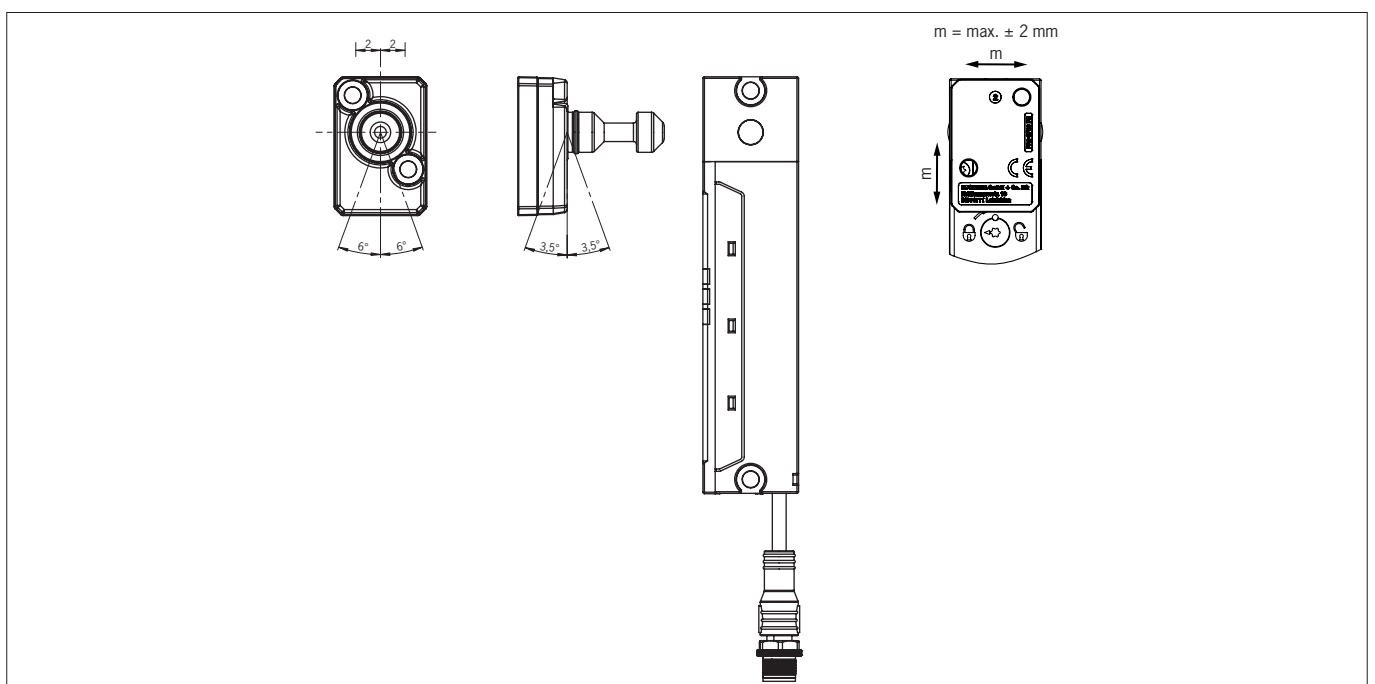
Fig. 4: Maximum actuator deflection and maximum center offset
