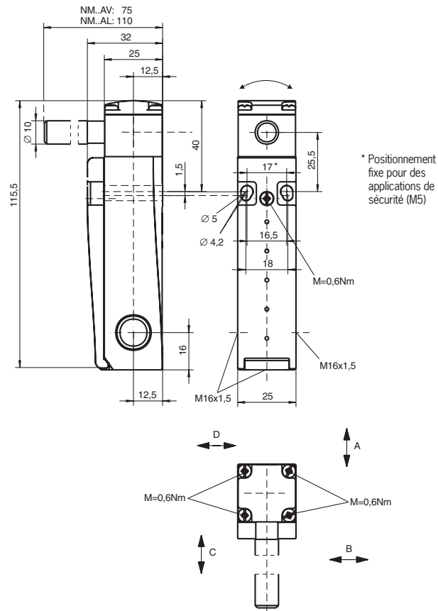
Fig. 5 : Dimensions NM11AV / NM02AV / NM12AV / NM03AV et NM11AL / NM02AL / NM12AL / NM03AL
