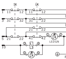
TZ.BHA...C1902 (com conector BHA12)
