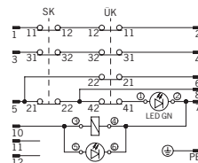
TZ.BHA...RC1924 (com conector BHA12)
