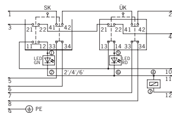
TZ.BHA...C1781 (com conector BHA12)
