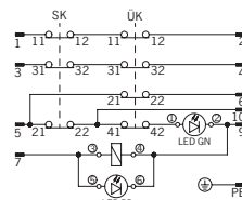
TZ.BHA...C1903/C2148/C2399 (com conector BHA12)
