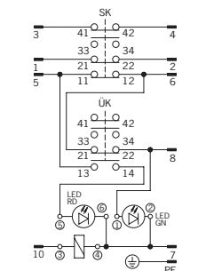
TZ.VABL12C-MF (com conector BHA12)
