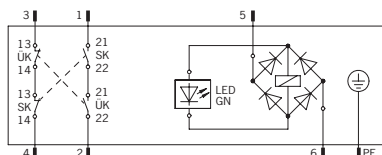
TZ...045177/045181/048492 (Com conector SR6)
