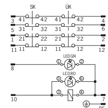
TZ.BHA...RC2408 (com conector BHA12)
