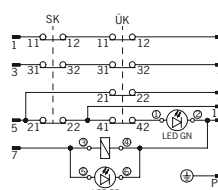
TZ..BHA...C1903/C2148/C2399 (s konektorom BHA12)
