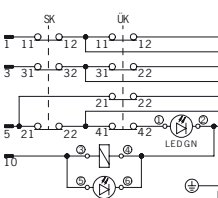
TZ..BHA...C1902 (s konektorom BHA12)
