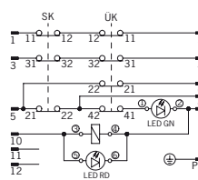
TZ..BHA...RC1924 (s konektorom BHA12)
