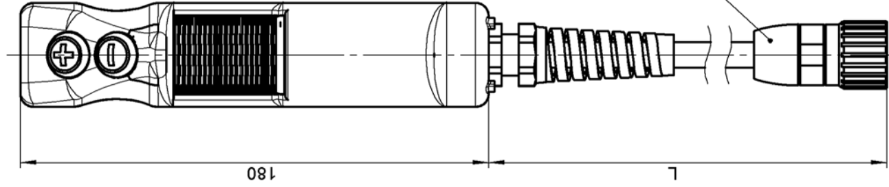
12-pol. Steckverbinder (Fa. Coninvers) 12-pin plug connector (Type Coninvers)
