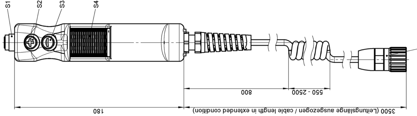
12-pol. Steckverbinder (Fa. Coninvers) 12-pin plug connector (Type Coninvers)
