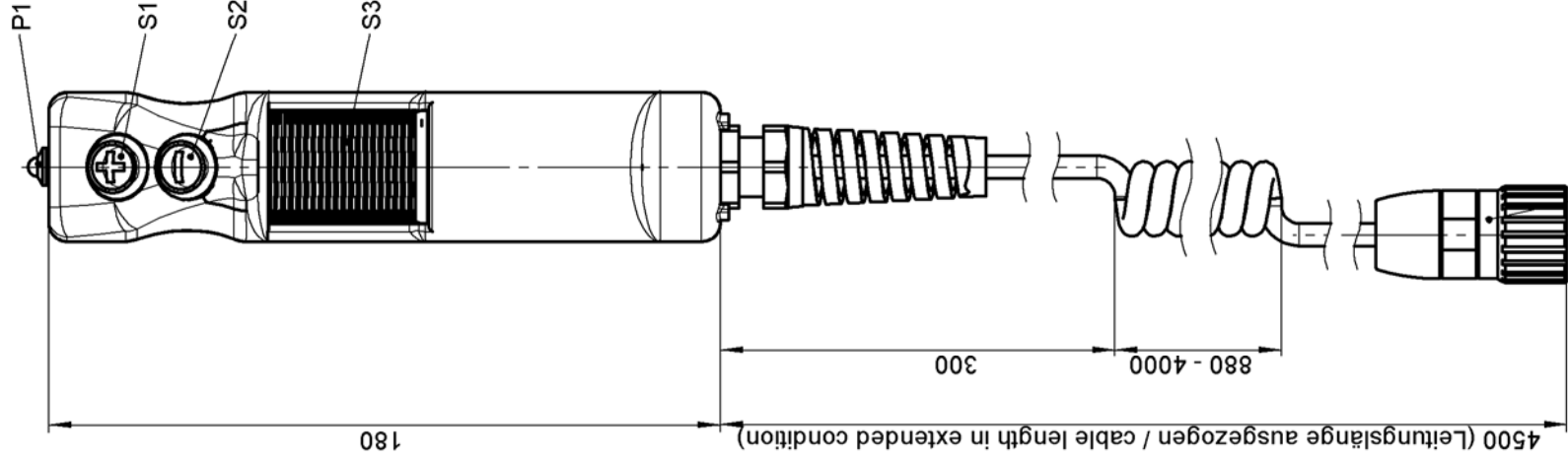
12-pol. Steckverbinder (Fa. Coninvers) 12-pin plug connector (Type Coninvers)
