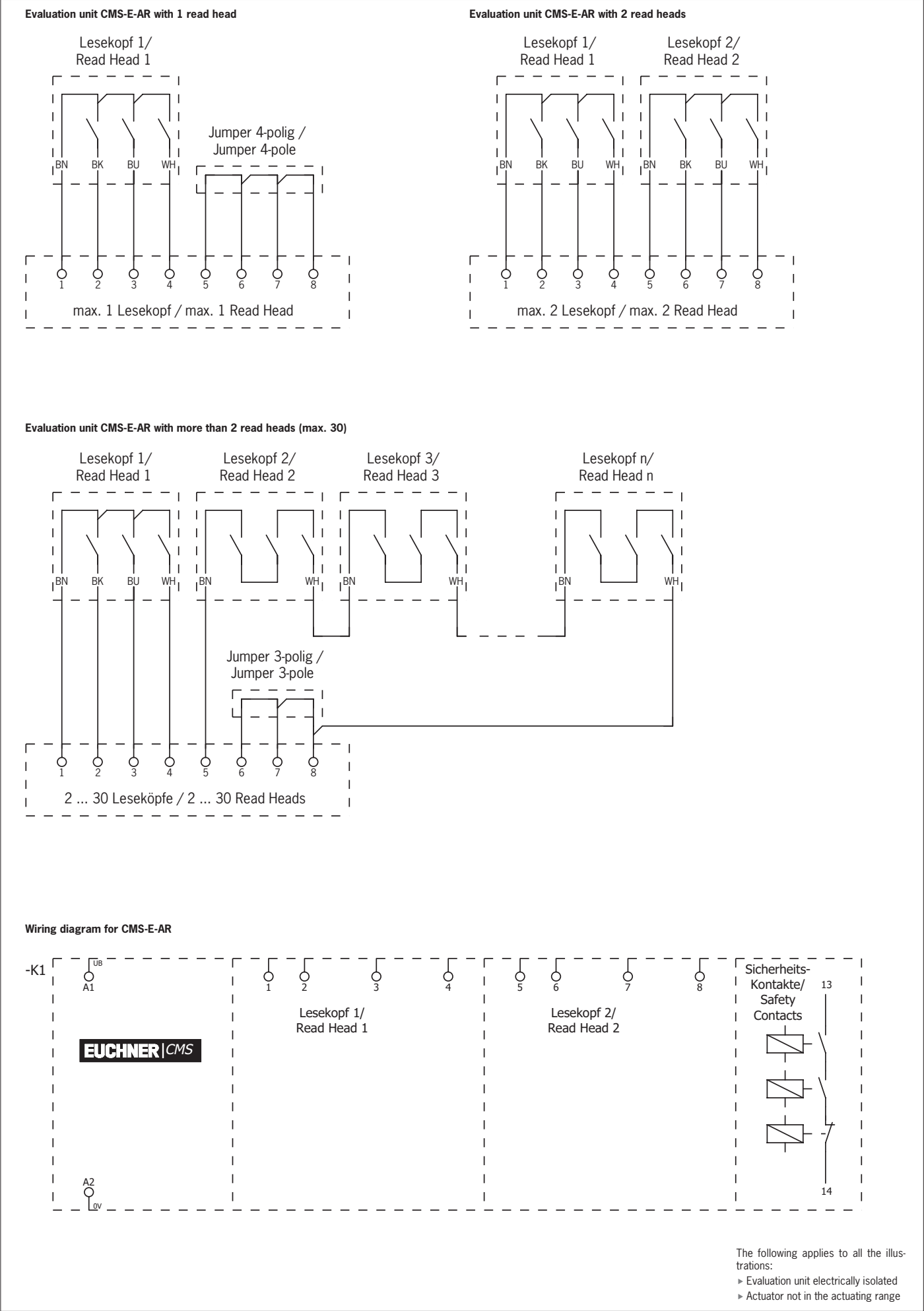
Fig. 2: Wiring diagram for CMSE-AR
