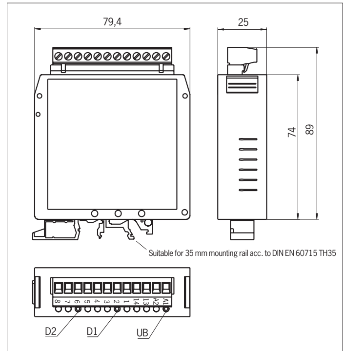
Fig. 1: Dimension drawing for evaluation unit CMS-E-AR
